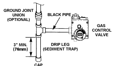
FIGURE 9 GAS PIPING WITH ALL BLACK IRON PIPE TO GAS CONTROL.
